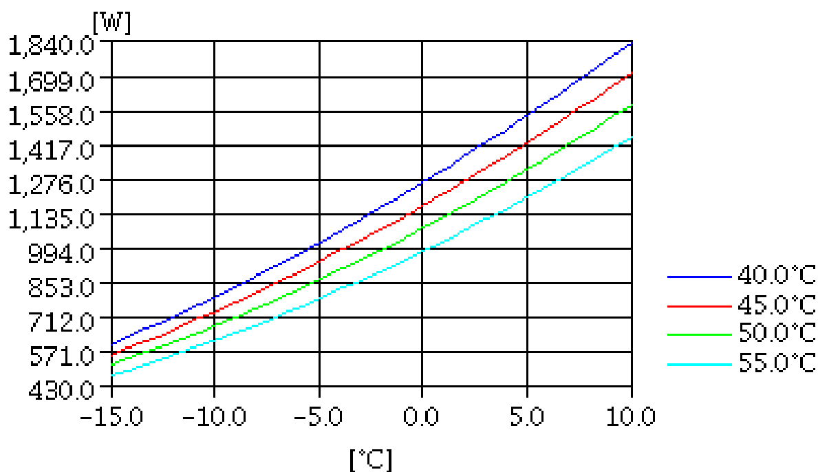
COOLING CAPACITY
