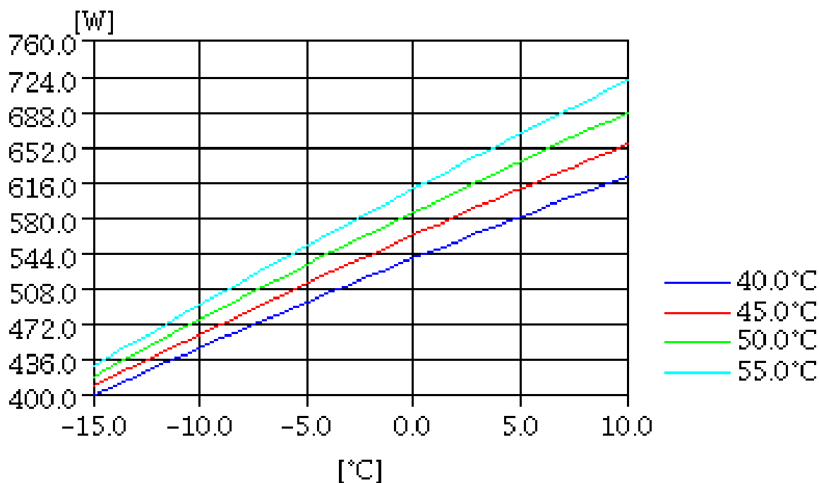
COOLING CAPACITY
